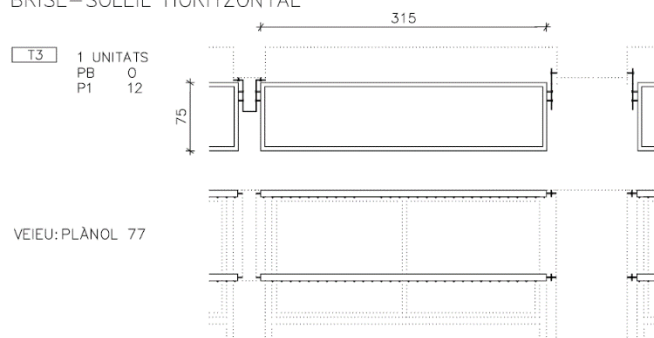
BRISE-SOLEIL HORIZONTAL
