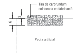
Detail carborundum
