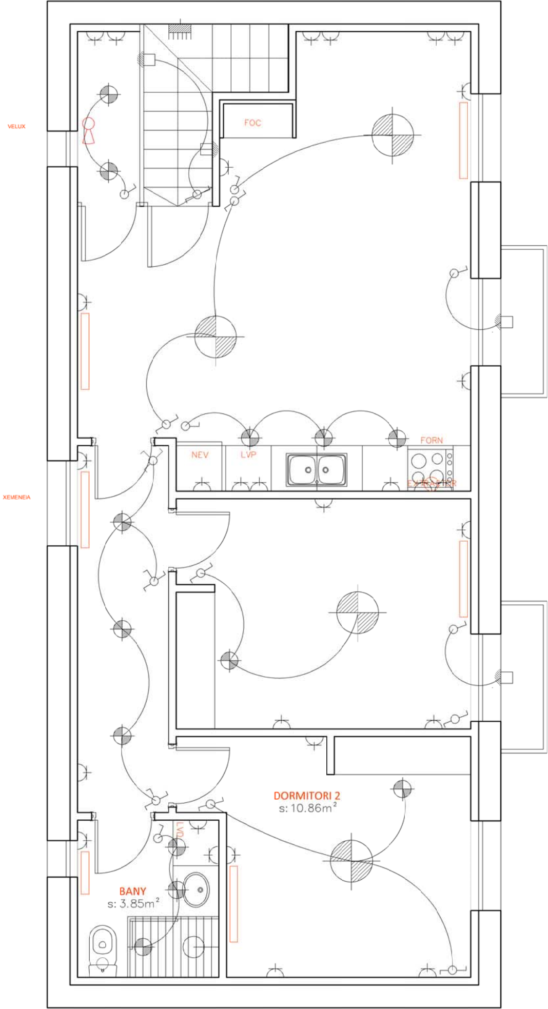
PLANOL ELECTRIC
