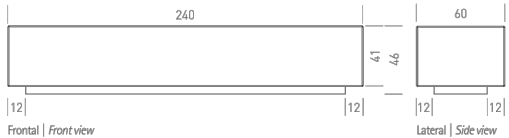
Frontal | Front view Peso | Weight: 1200 kg
