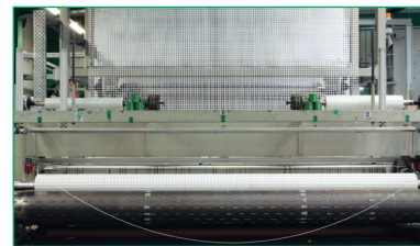
Figure 11 Secugrid® production
