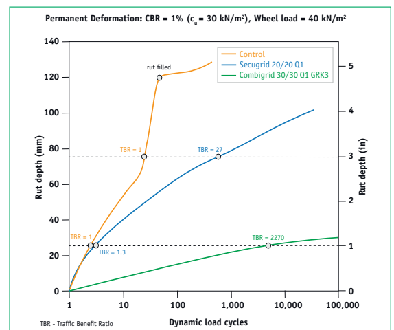
Figure 6: Combigrید® and Secugrid® traffic benefit ratio (TBR) over a very weak subsoil, compared to an unreinforced section (for subsoils CBR 1%, for details see EuroGeo4, paper 229)
