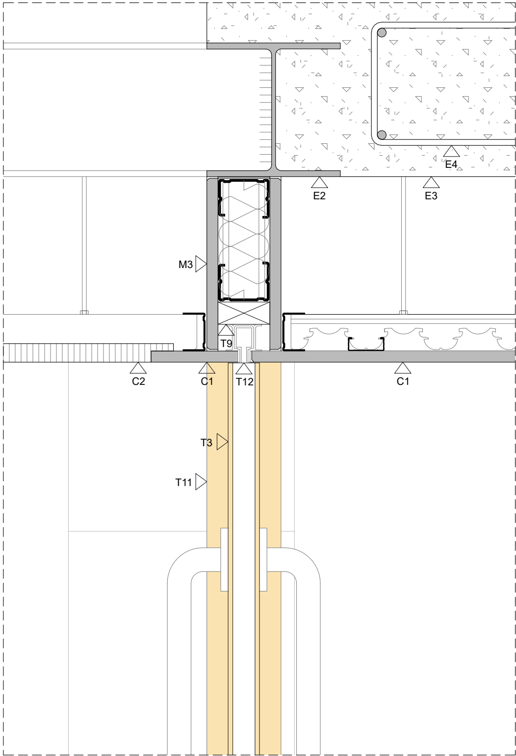
DETALL 06.1
