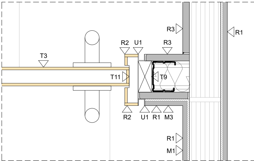
DETALL 04.3
