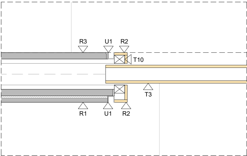
DETALL 04.2
