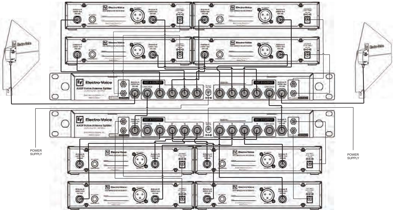
Patching an 8-channel system
