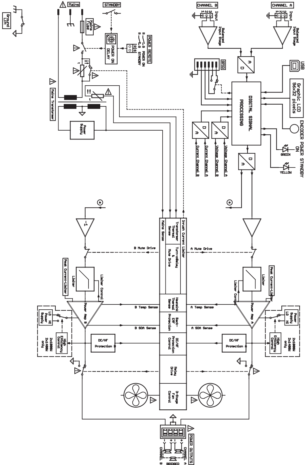
Block diagram
