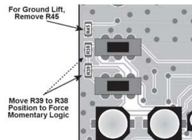
Figure 3: PC Board Detail
