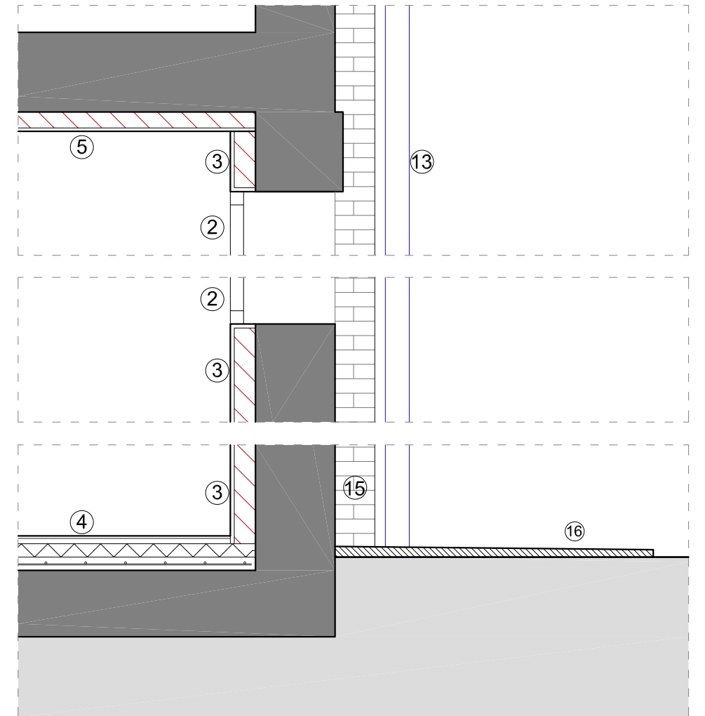
DETALL PAVIMENT SALA POLIVALENT
