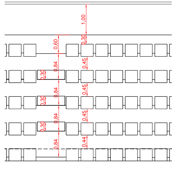
DETALL GRADES esc 1/75
