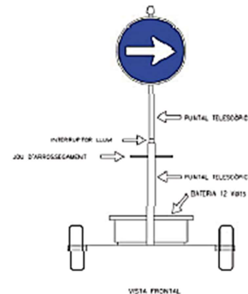
VISTA FRONTAL
