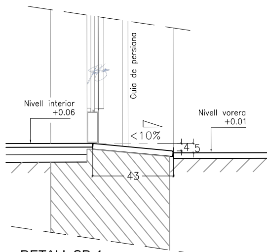
DETALL SD-1 E: 1/20
