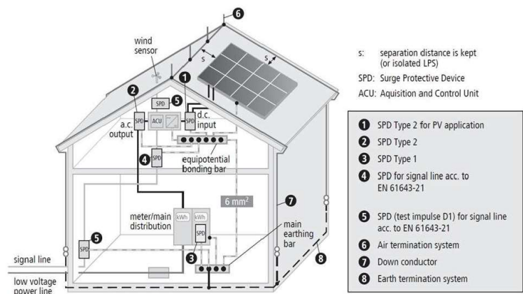
Figure 4 – Installation of SPDs in case of a building with external LPS when separation distance s is kept – Installation with data acquisition and control system
