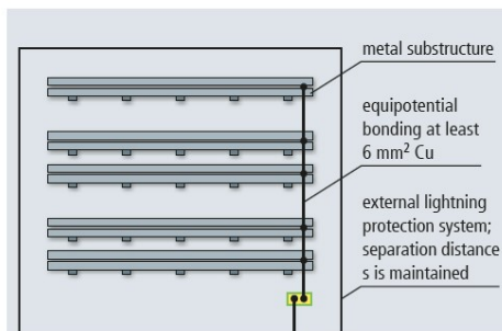
Figure 1 Functional earthing of the mounting systems if no external lightning protection system is installed or the separation distance is maintained (DIN EN 62305-3, Supplement 5)
